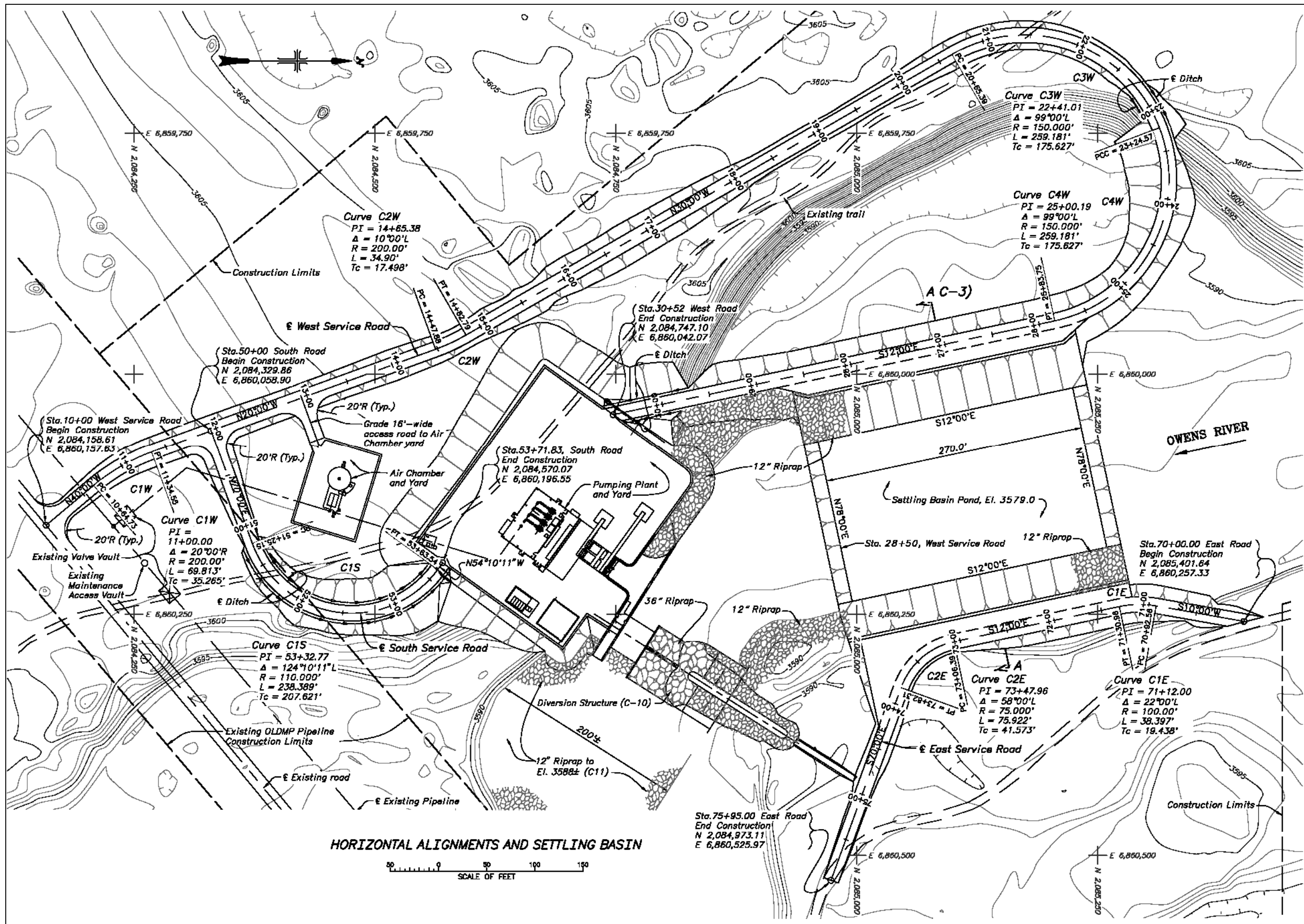
Figure 2-7. Overview of Diversion and Pump Station
