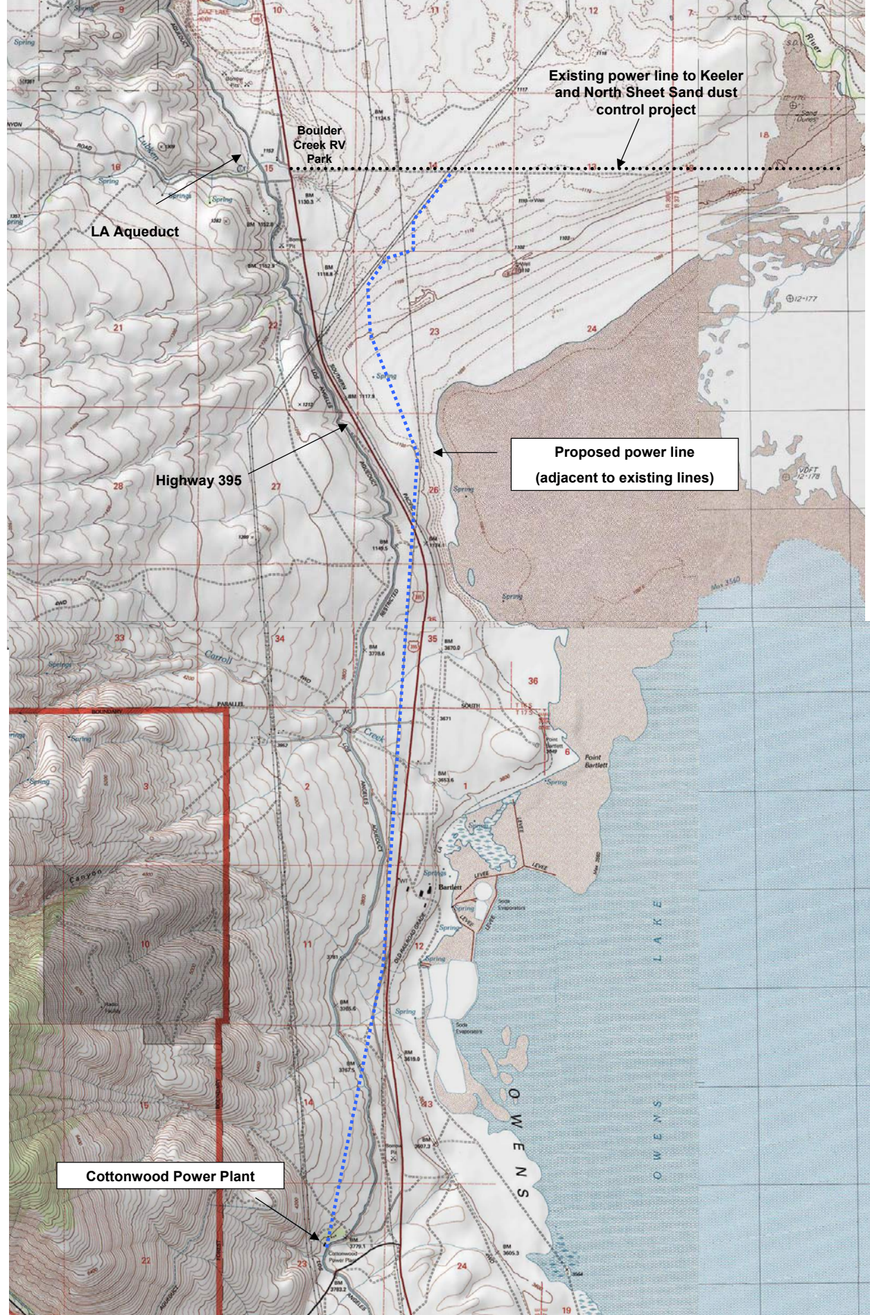
Fig. 6-10 Proposed Power Line
