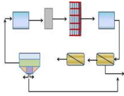
Process Water Recycling System Diagram
