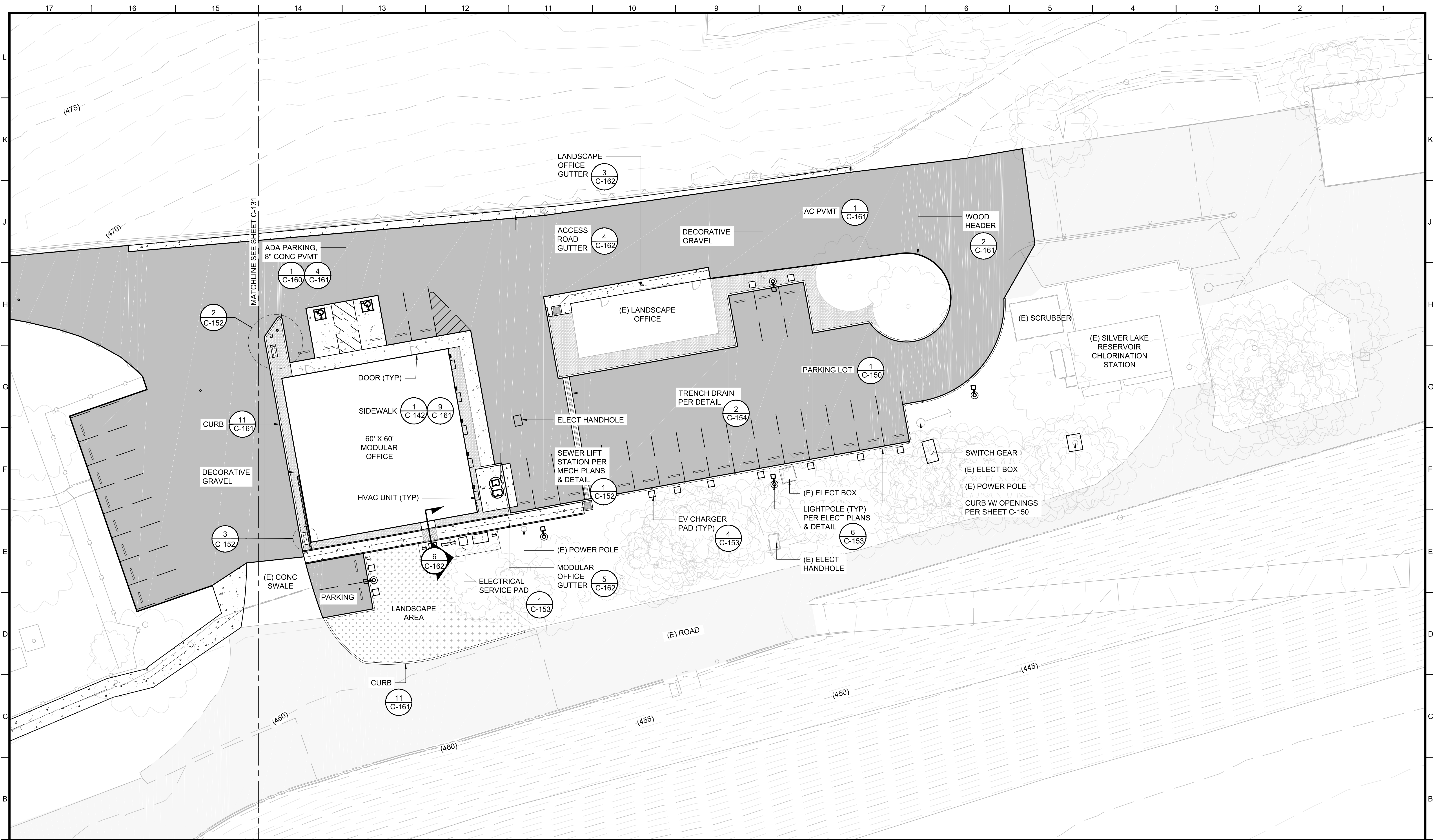
SITE PLAN - SOUTH 1 SCALE: 1" = 15'-0" C-130, C-131 C-132
