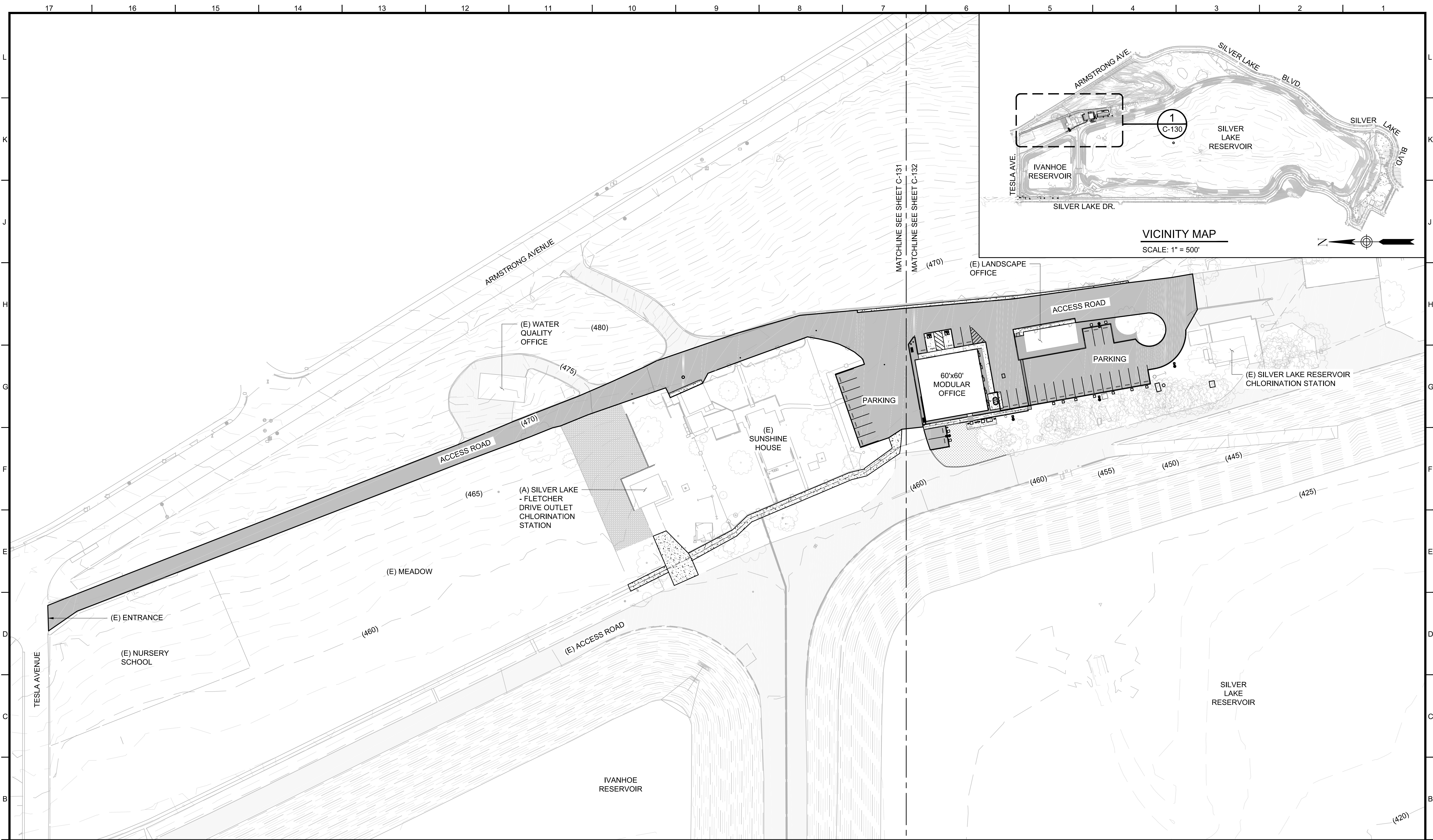
SITE PLAN SCALE: 1" = 40'-0"
