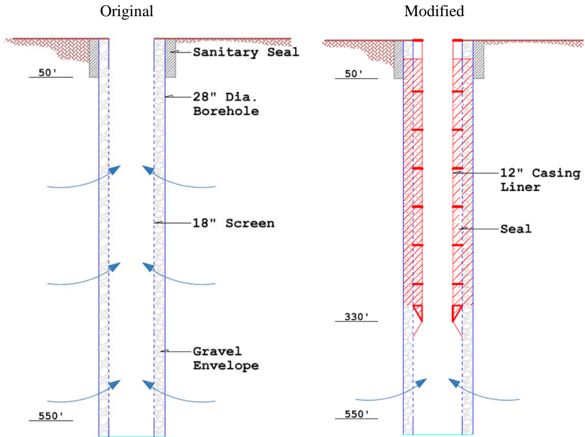
Figure 2 – Comparison of Original and Modified W385 Designs
